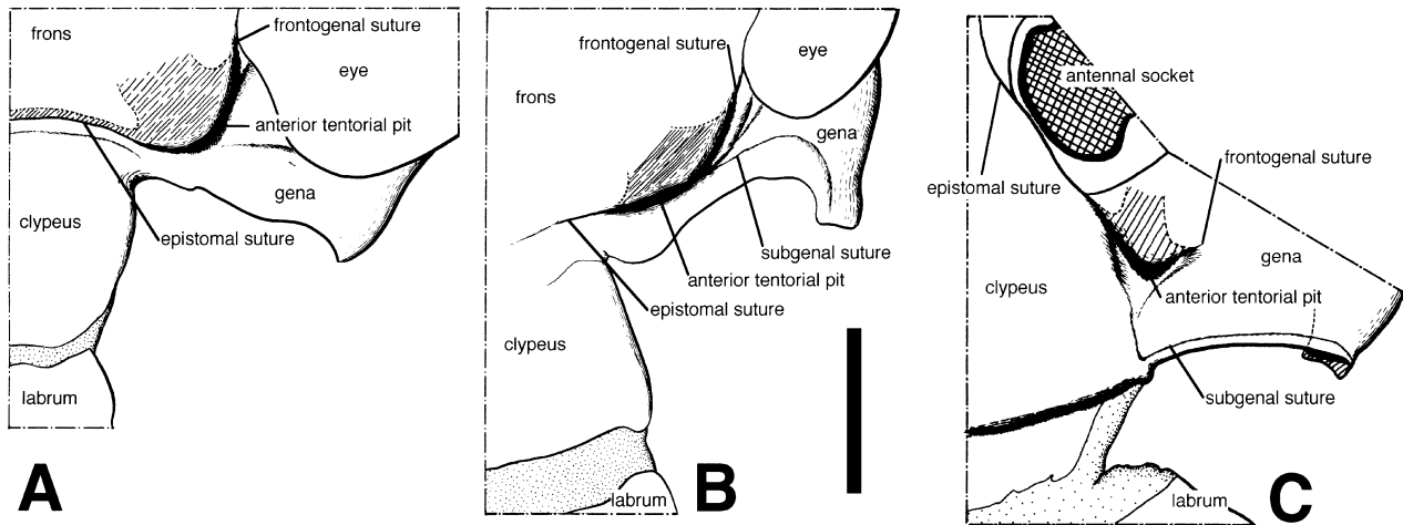
Fig. 2 —Anterior tentorial pit and surrounding structures — A. Acromantis japonica (Mantodea) — B. Pycnoscelus surinamensis (Blattodea) — C. Psococerasis nubila (Psocoptera). Scale = 0.5 mm.
