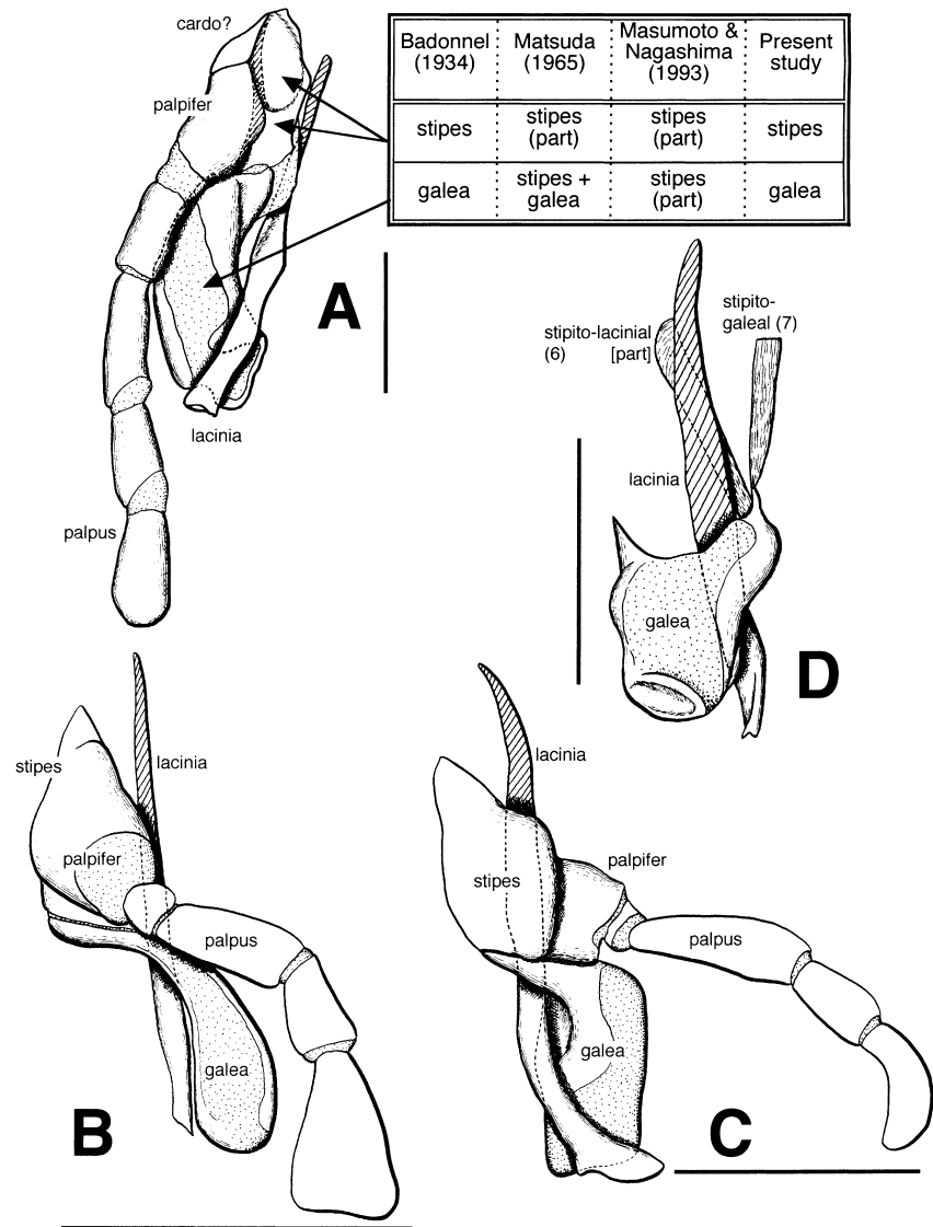
Fig. 4 —Maxilla — A. Psococerastis nubila (Psocomorpha: Psocidae), lateral aspect, with different interpretations of the maxilla of Psocoptera — B. Echmepteryx lunulata (Trogiomorpha: Lepidopsocidae), lateral aspect — C. Paramphientomum sp. (Troctomorpha: Amphientomidae), lateral aspect — D. ditto, showing muscles attached to galea and lacinia, anterior aspect. Scale = 0.5 mm.
